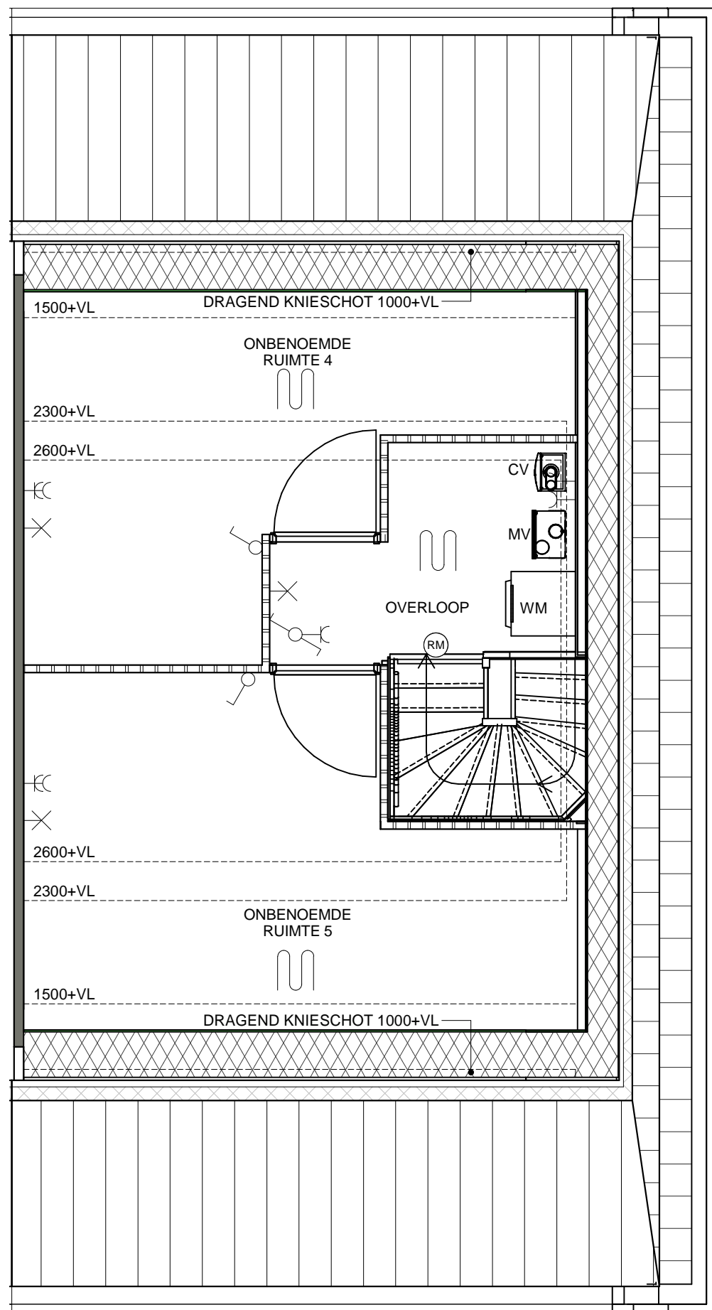
9301300_indeling zolder type C
